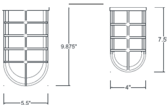
GU-1 CAST GUARD
