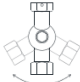
LGSWL 1/2" NPT swivel For all arms greater than 7" wide in diameter
