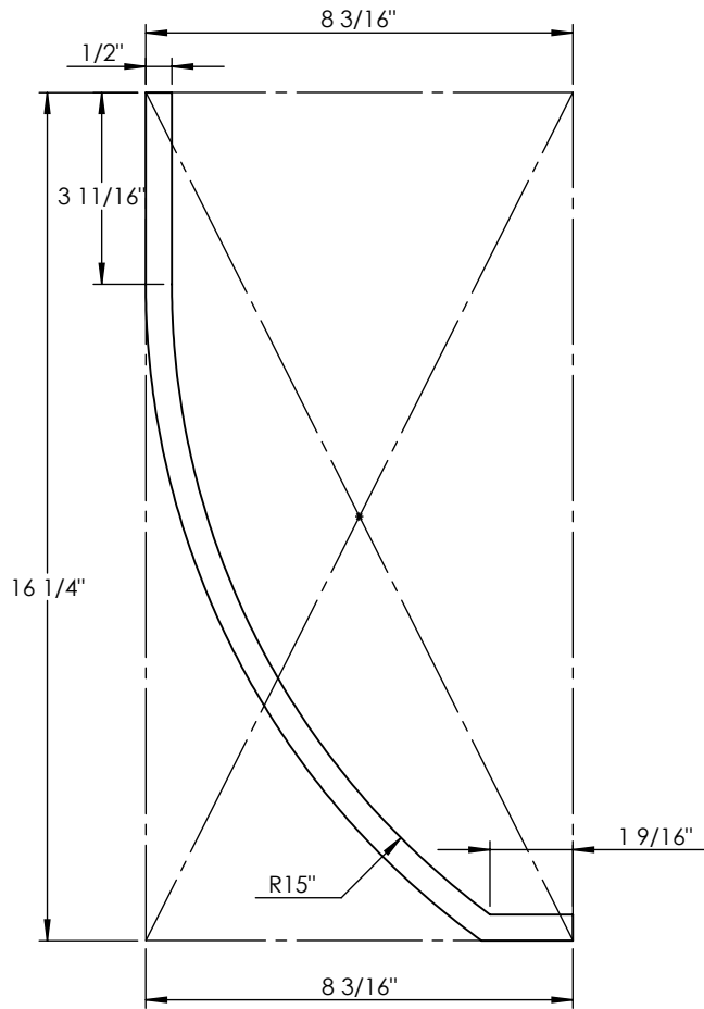
1" X 1/2" TUBE WITH LENGTH OF 18-1/8"
